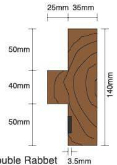
Double Rabbet
