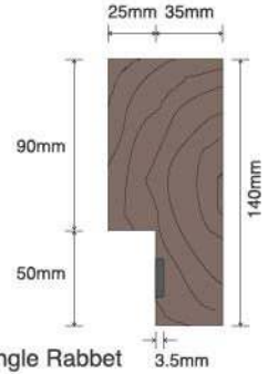
Single Rabbet
