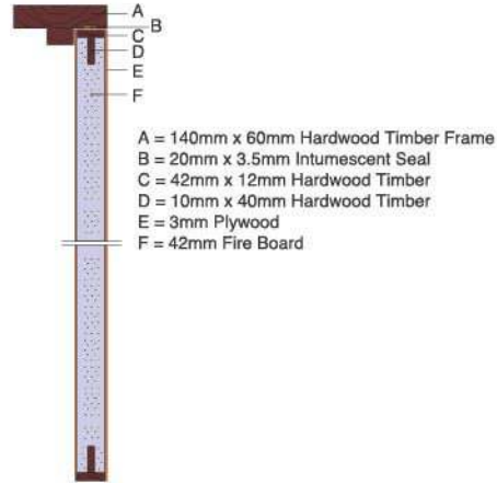
Single Rabbet
