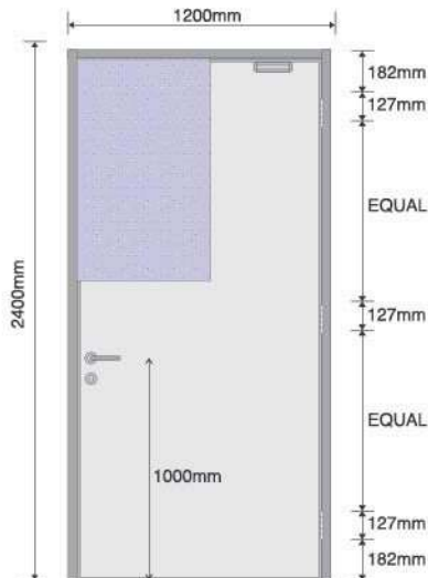
Front & Internal Elevation Of Doorset Model : Vulgaris
