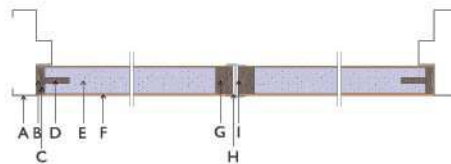
Horizontal Section Of Doorset
