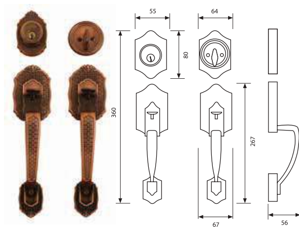
LOKRITE 400PE-US5-60MM DOUBLE HANDLESET LOCK 152L-400PE05BP
