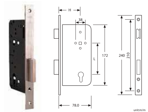
LOKRITE ME-L-60-DL-STS DEAD-LOCKCASE (60MM BACKSET) & SS FACE PALTED 152GM-L-60DLSTS
