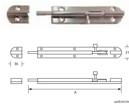
LOKRITE H01-002 SS Box Flushbolt size 150 x 20mm 152G-BFB150S
