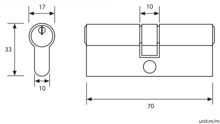
LOKRITE SN LA1-70MM KEY THUMBTURN PROFILE CYLINDER (E02-007) 152GM-LA1
