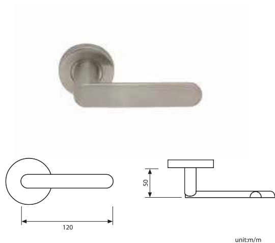
LOKRITE SF002 SS SOLID LEVER HANDLE WITH ROUND ROSE & PROFILE CYLINDER ESCUTCHEON ROSE 152L-SF-002
