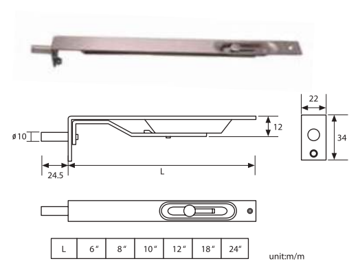
LOKRITE 300 x 22mm Stainless Steel Flush Bolt 152L-FB300S
