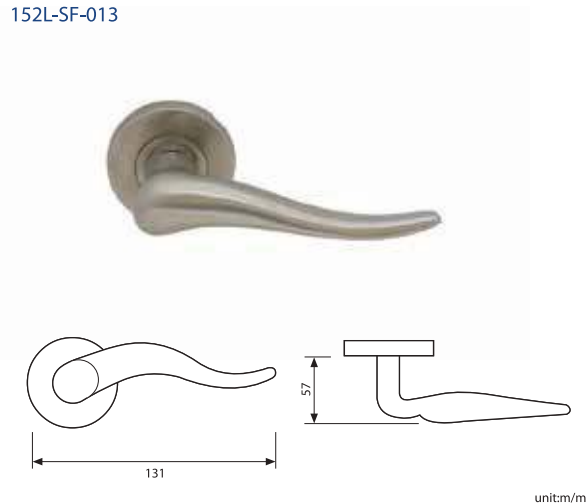
LOKRITE SF013 SS SOLID LEVER HANDLE WITH ROUND ROSE & PROFILE CYLINDER ESCUTCHEON ROSE 152L-SF-013
