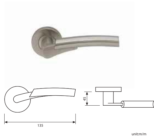
LOKRITE SF008 SS SOLID LEVER HANDLE WITH ROUND ROSE & PROFILE CYLINDER ESCUTCHEON ROSE 152L-SF-008
