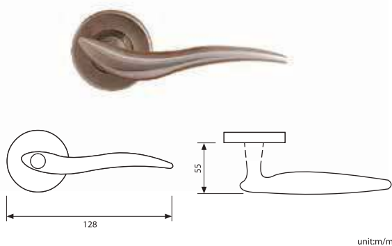
LOKRITE SF052 SS SOLID LEVER HANDLE WITH ROUND ROSE & PROFILE CYLINDER ESCUTCHEON ROSE 152L-SF-052
