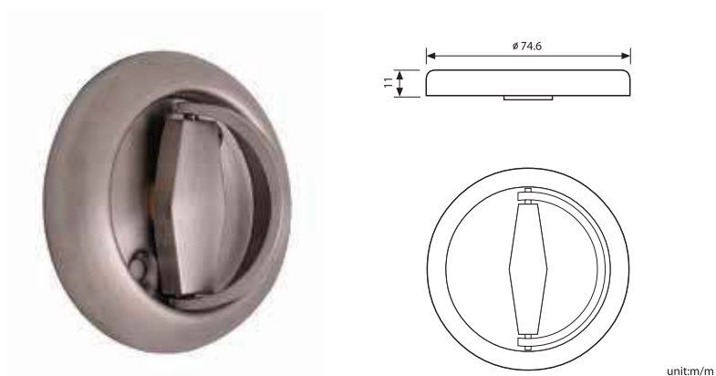
LOKRITE LE-08001 SS Flush Pull Ring with screws 152G-LE-08001
