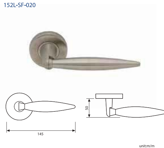
LOKRITE SF020 SS SOLID LEVER HANDLE WITH ROUND ROSE & PROFILE CYLINDER ESCUTCHEON ROSE 152L-SF-020
