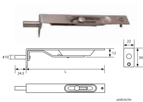
LOKRITE 150 x 22mm Stainless Steel Flush Bolt 152L-FB150S
