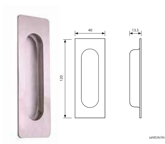
LOKRITE Oval Shape SS Flush Pull D03-003 152G-PS03
