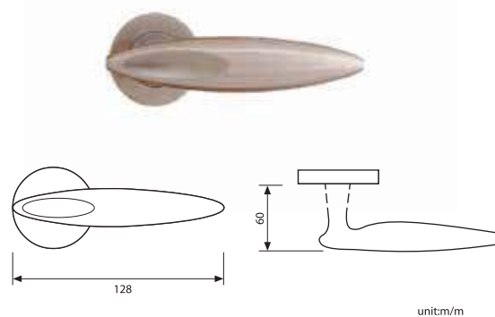
LOKRITE SF146-RH SS SOLID LEVER HANDLE WITH ROUND ROSE & PROFILE CYLINDER ESCUTCHEON ROSE (Right Hand) 152L-SF-146LH
