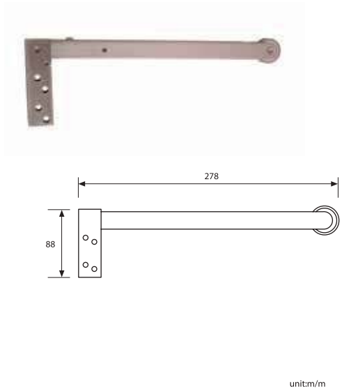
LOKRITE LE-6001 STAINLESS STEEL DOOR SELECTOR 152L-LE-6001
