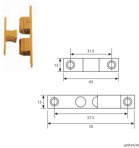
LOKRITE 70MM DBRASS BALL CATCH 10-S1-254 152G-K05-005
