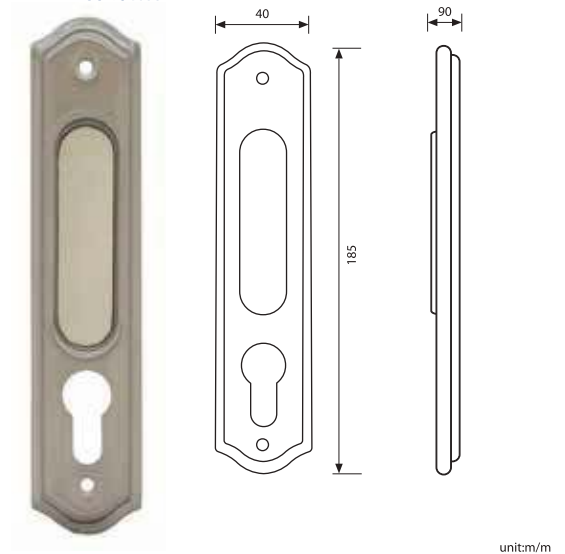
LOKRITE Flush Pull with profile cylinder hole in SN finish 147-AS540WH
