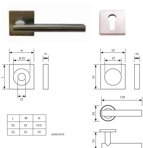
LOKRITE SS LEVER HANDLE SF031+GT09+GT04 SQUARE ROSE AND ESCUTCHEON ROSE 152L-SF031GT09GT04
