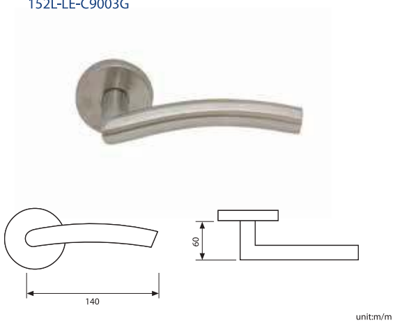
LOKRITE SD010 SS TUBULAR LEVER HANDLE WITH ROUND ROSE & PROFILE CYLINDER ESCUTCHEON ROSE 152L-LE-C9003G
