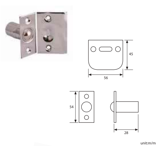
LOKRITE K05-002 CP ROLLER BALL CATCH WITH SCREWS 152G-K05-002
