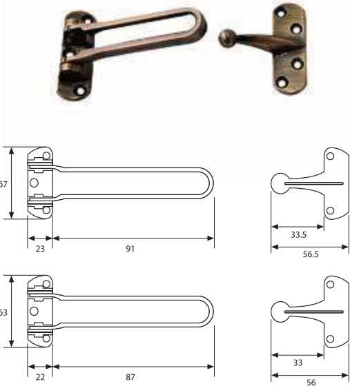
LOKRITE 10-G1-302-US5 DOOR GUARD 152L-10G1302-05
