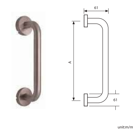
LOKRITE LE-CH22G Stainless Steel D Pull Handle with screws size 200 x 19mm 152G-C11-002
