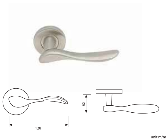
LOKRITE SF007 SS SOLID LEVER HANDLE WITH ROUND ROSE & PROFILE CYLINDER ESCUTCHEON ROSE 152L-SF-007
