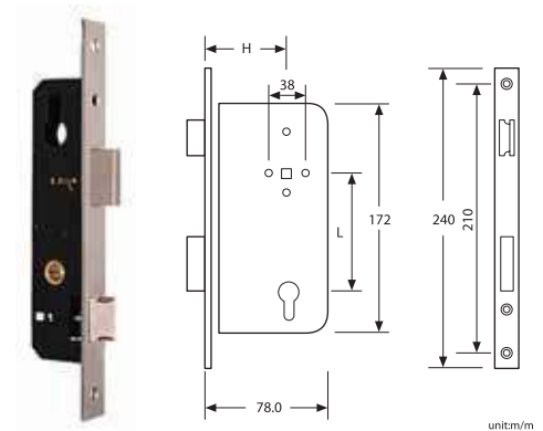
LOKRITE LC-NP NARROW MORTISE LOCKCASE 22 x 85MM 152L-LC09
