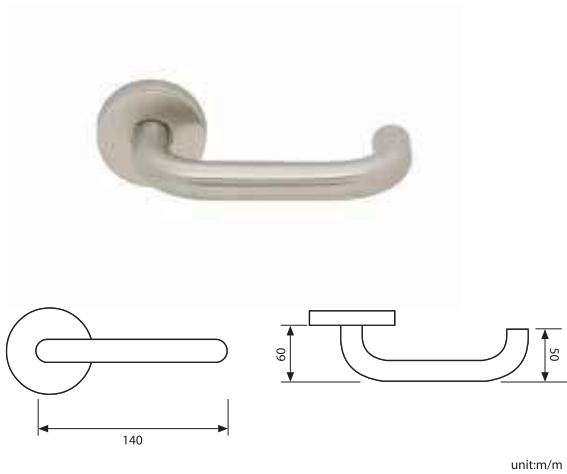
LOKRITE SD001 SS TUBULAR LEVER HANDLE WITH ROUND ROSE & PROFILE CYLINDER ESCUTCHEON 152L-LE-C9003G
