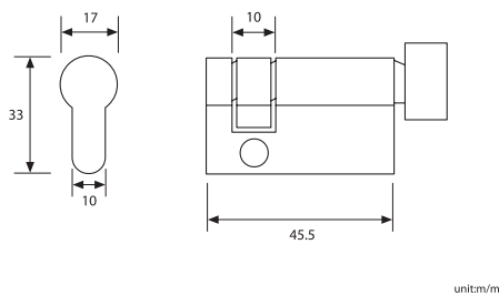
LOKRITE HALF PROFILE CYLINDER TT BLANK (ME-L-A12B) 152L-ME-L-A12B
