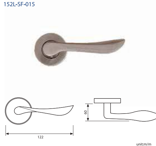
LOKRITE SF015 SS SOLID LEVER HANDLE WITH ROUND ROSE & PROFILE CYLINDER ESCUTCHEON ROSE 152L-SF-015
