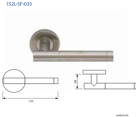
LOKRITE SF035 SS SOLID LEVER HANDLE WITH ROUND ROSE & PROFILE CYLINDER ESCUTCHEON ROSE 152L-SF-035
