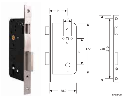
LOKRITE MORTISE LOCKCASE 60 x 85 MM & 240 MM STRIKE PLATE 152GM-LC
