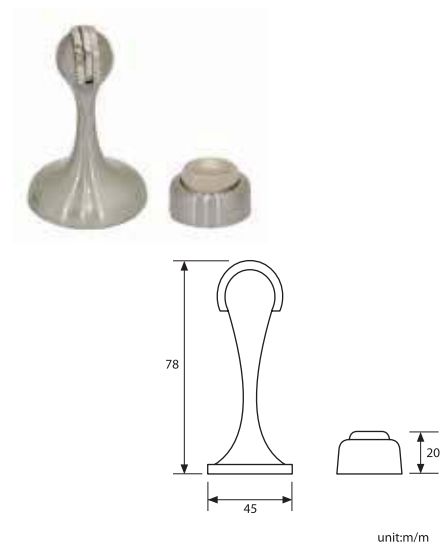
LOKRITE F03-005-PB MAGNETIC DOOR STOP 152G-F03-00515
