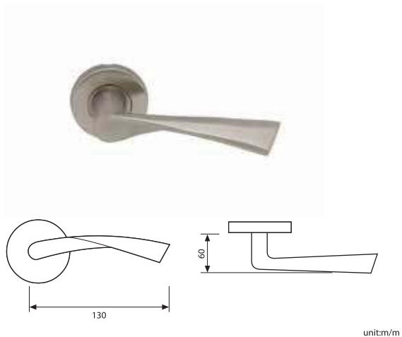
LOKRITE SF001 SS SOLID LEVER HANDLE WITH ROUND ROSE & PROFILE CYLINDER ESCUTCHEON ROSE 152L-SF-001
