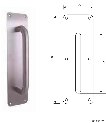
LOKRITE LE-PH-305G 200 x 19mm diameter Pull Handle on 306 x 75 x 1.5mm thick Back Plate with screws 152G-LE-PH-305G
