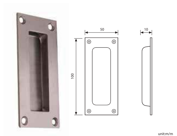
LOKRITE SS Flush Pull with screws size 100 x 50mm D03-004 152G-PS04
