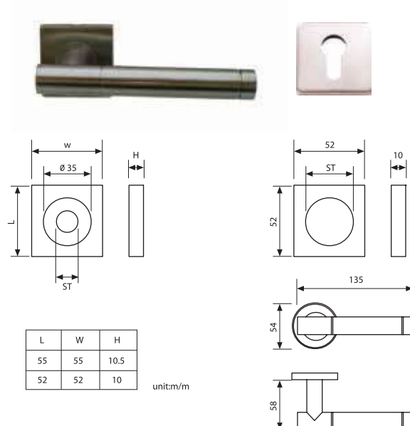
LOKRITE SS LEVER HANDLE SF035+GT09+GT04 SQUARE ROSE AND ESCUTCHEON ROSE 152L-SF035GT09GT04
