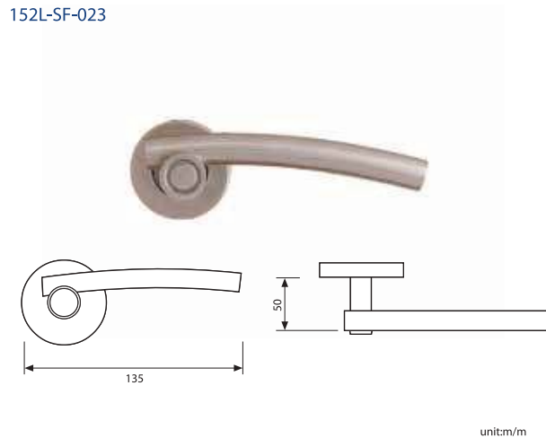
LOKRITE SF023 SS SOLID LEVER HANDLE WITH ROUND ROSE & PROFILE CYLINDER ESCUTCHEON ROSE 152L-SF-023
