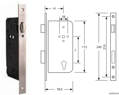
LOKRITE MORTISE LOCKCASE WITH SPRING LOADED DOUBLE ACTION LATCH 60 x 85 MM 152GM-LC-E01-003
