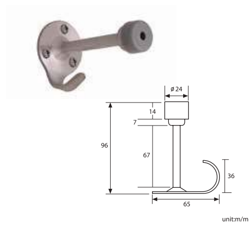
LOKRITE 8800 SS HAT & COAT HOOK DOOR STOP WITH GREY RUBBER 152G-8800
