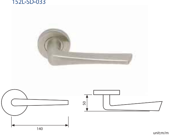
LOKRITE SD033 SS TUBULAR LEVER HANDLE WITH ROUND ROSE & PROFILE CYLINDER ESCUTCHEON ROSE 152L-SD-033
