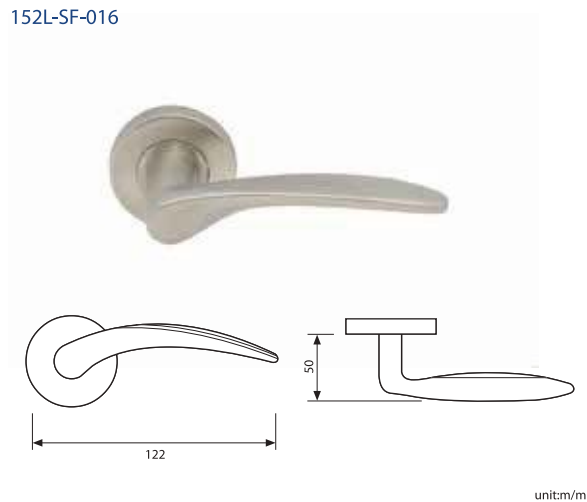
LOKRITE SF016 SS SOLID LEVER HANDLE WITH ROUND ROSE & PROFILE CYLINDER ESCUTCHEON ROSE 152L-SF-016
