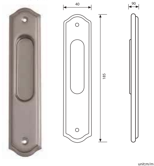
LOKRITE Flush Pull without profile cylinder hole in satin nickle finish 147-AS540NH
