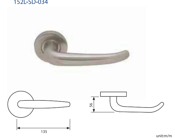
LOKRITE SD034 SS TUBULAR LEVER HANDLE WITH ROUND ROSE & PROFILE CYLINDER ESCUTCHEON ROSE 152L-SD-034
