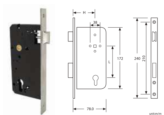
LOKRITE MORTISE LOCKCASE LC01-PS PASSAGE SINGLE ACTION 152L-LC01PS
