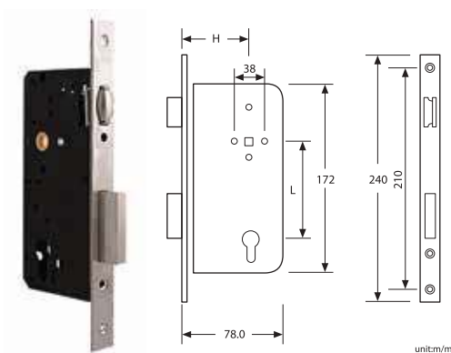
LOKRITE PASSAGE MORTISE LOCKCASE 60 x 85 MM WITH ROLLER LATCH & 240MM STRIKE PLATE AND DEADBOLT 152GM-LC-E01-003
