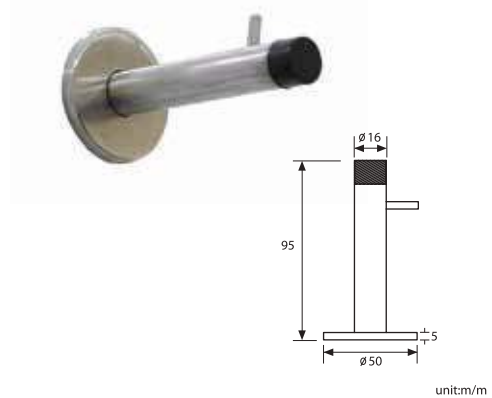
LOKRITE SSS DOOR STOP WITH HAT & COAT HOOK (SYA-04) 152L-SYA-04
