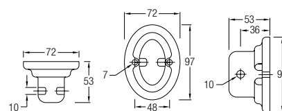
DOUBLE TOWEL RAIL 915MM WBSLTR000WW
