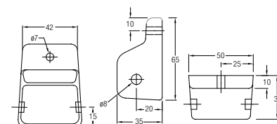
TOILET ROLL HOLDER WITH SHELF WBSSTH000WW
