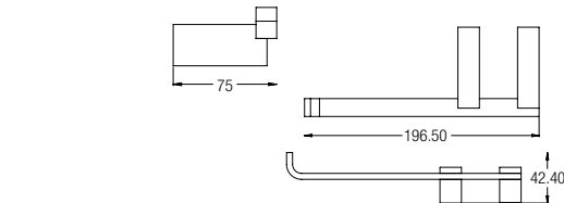
SOAP DISPENSER WBBA100251CP
