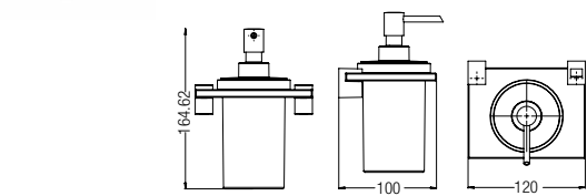
GLASS SHELF & TUMBLER WBBA100250CP
