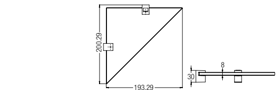
GLASS SHELF 600MM WBBA100248CP
