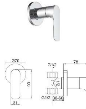
191.08101 CP brass 1/2" concealed stopcock with quarter turn single lever handle and sliding wall flange.
