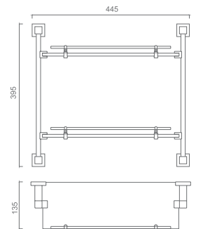
17416 Double glass shelf Material: Brass Finish: Chrome
