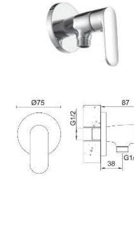
175.03101 CP brass 1/2" angle valve with quarter turn single lever handle and wall flange.
