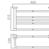
181142 Towel rack Material: Brass Finish: Chrome
