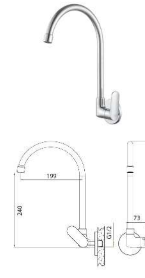
175.08101 CP brass wall mounted sink tap with quarter turn single lever handle, swivel spout and wall flange.
