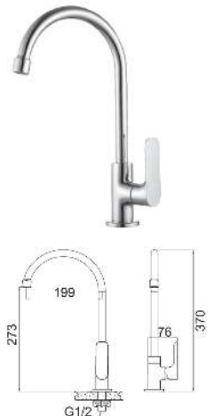
191.03101 CP brass pillar sink tap with quarter turn single lever handle and swivel spout.
