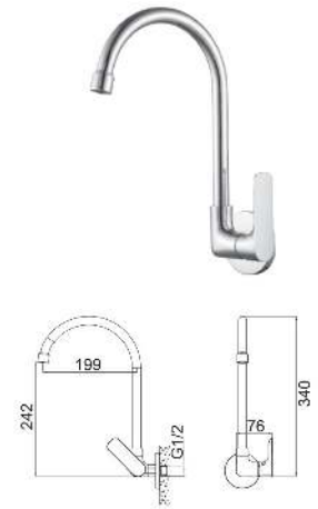
191.04101 CP brass wall mounted sink tap with quarter turn single lever handle, swivel spout and wall flange.
