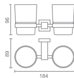
17402 Double cups holder Material: Brass Finish: Chrome
