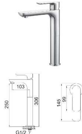
191.02101 CP brass tall basin pillar tap with quarter turn single lever handle.
