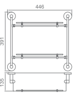
18116 Double glass shelf Material: Brass Finish: Chrome
