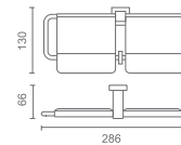
1741012 Tissue holder Material: Brass Finish: Chrome
